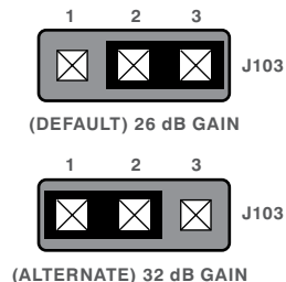
FIGURE 2: Close-up of J103 settings for the Model 501
