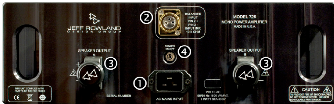
Figure 2: Rear Panel
